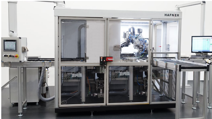
The measurement and testing machine for truck brake discs allows for 100% controlling, detects even the smallest errors, and precisely measures diameters, lengths and dimensional tolerances.
