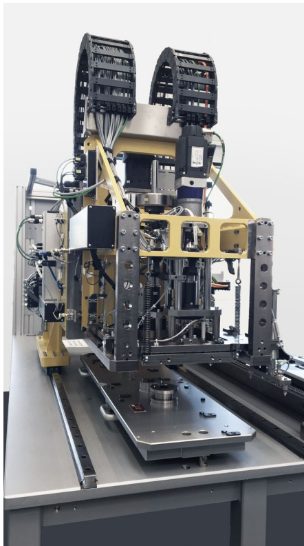
The solution for E-gears measures adjusting washers and sealing profiles, as well as the thickness of washers and sealing profiles on gears and housings, including adjusting washer magazine.
