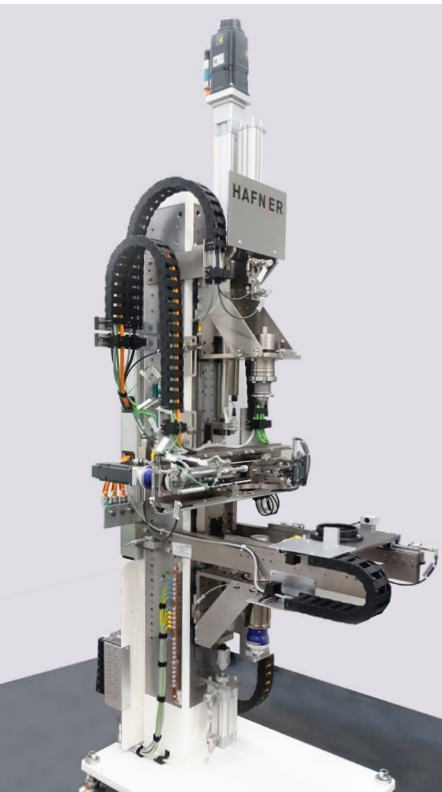
Vertical ShaftControl offers high flexibility for precisely checking all rotationally symmetrical workpieces. It is available in different versions, and can be optimally adjusted to custom requirements.
