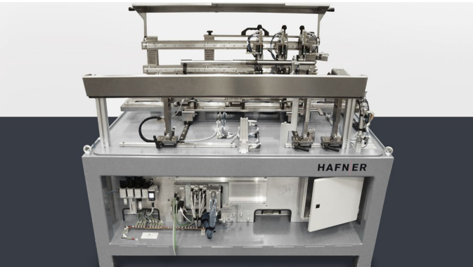
The post-process measuring machine for racks conducts tactile and dynamic measurements of the diameter of the ball screw track and thread pitch.
